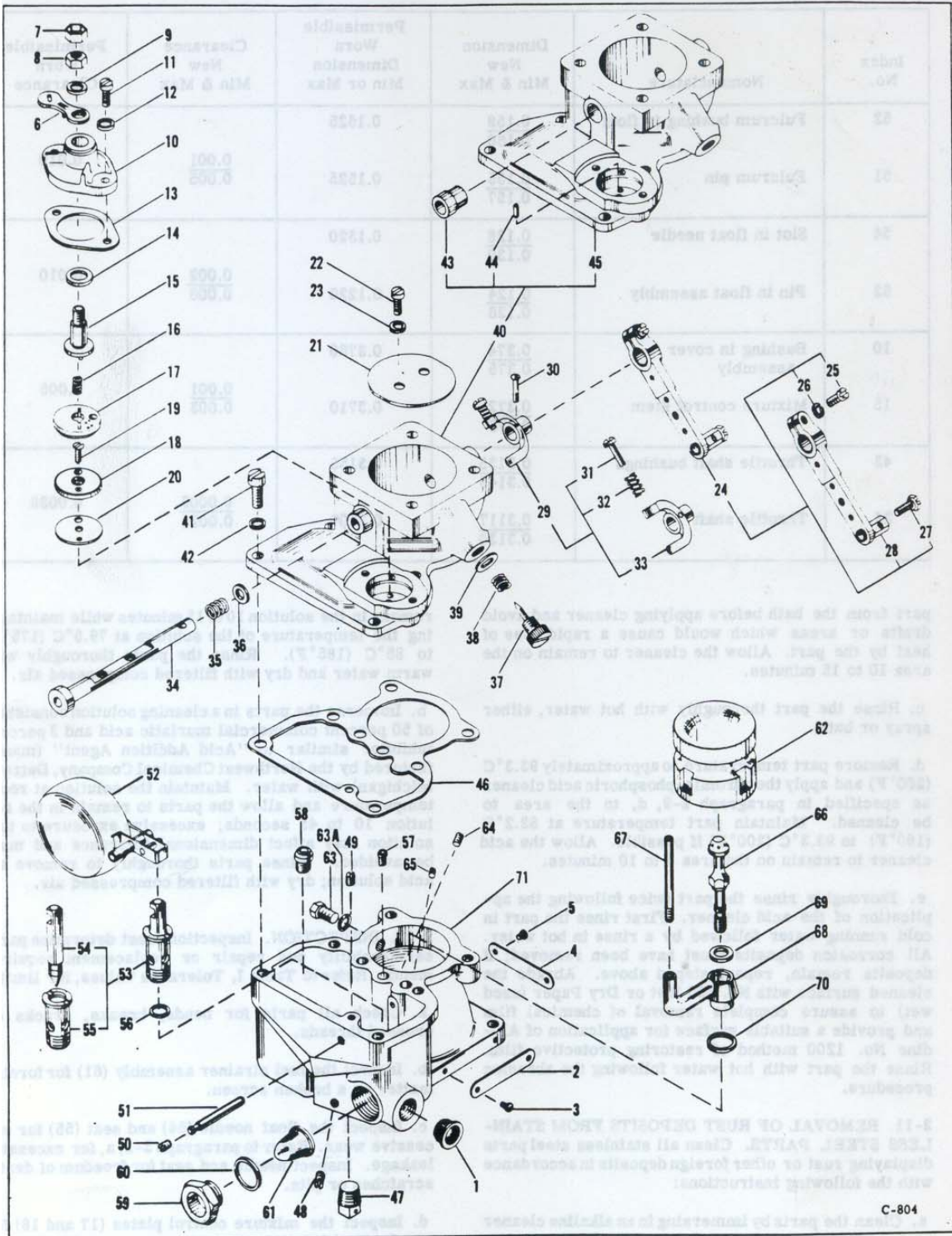
Figure 2-4. Exploded View of Stromberg NA-33A1 Float Carburetor
