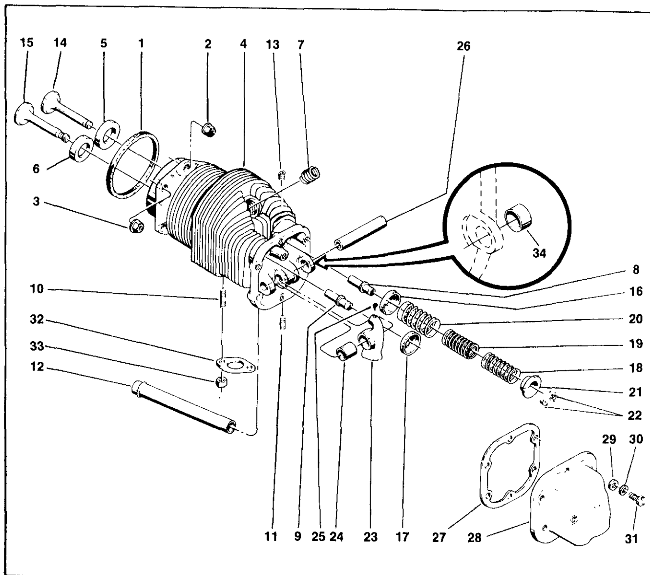
FIGURE 9. CYLINDER ASSEMBLY
