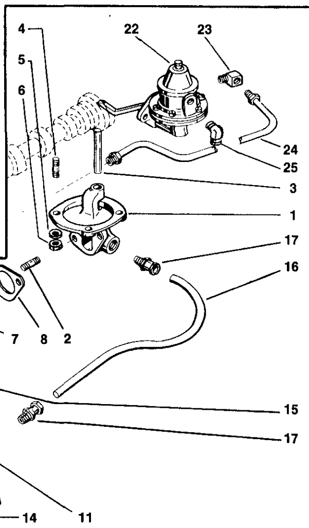
FIGURE 18. FUEL PUMP EQUIPMENT
