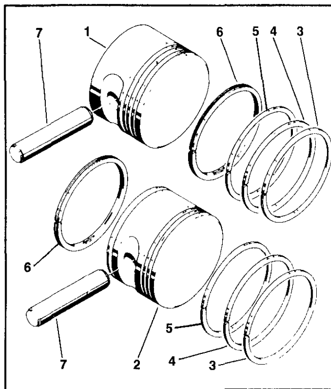
FIGURE 7. PISTON ASSEMBLY
